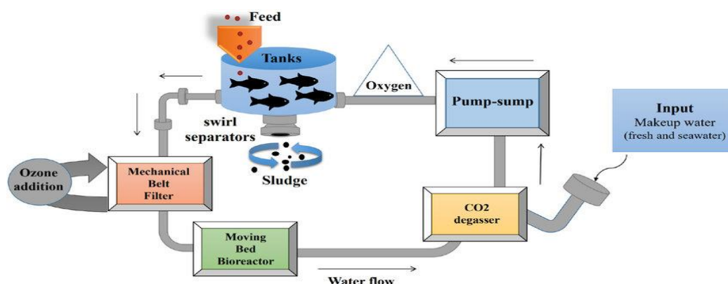
Fig 1: Recirculating Aquaculture System
