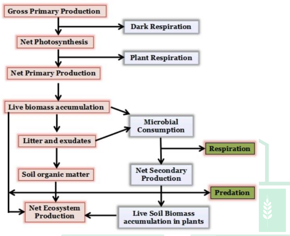
Fig 1. Mechanism of carbon sequestration
