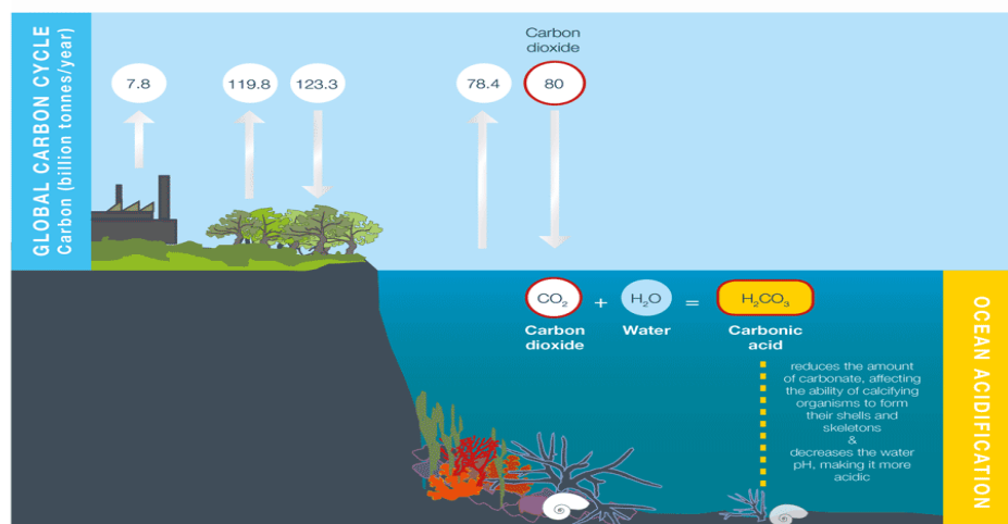
Figure 1: CO 2 emissions from various ecosystems. Source: Adapted from J. Cook, skepticalscience.com .
