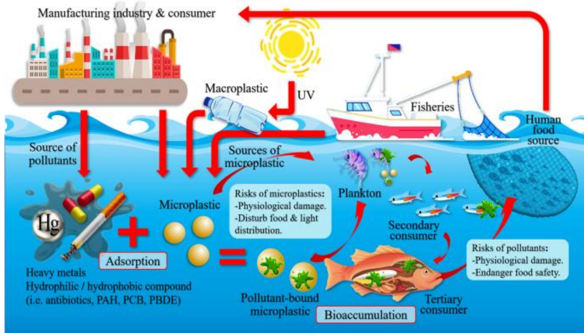
Fig 1: Microplastics in Ocean
